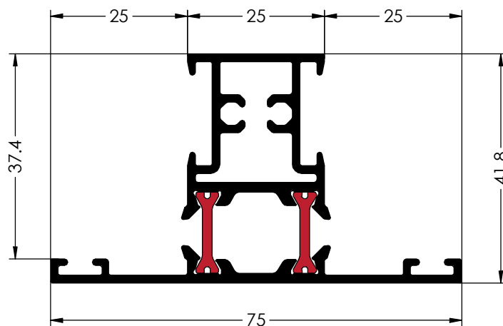
Ref. 9886 PILASTRA
